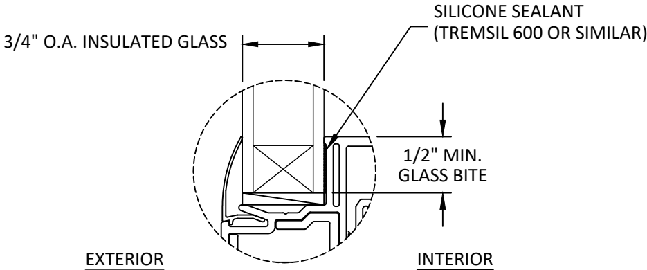
GLAZING DETAIL 1
