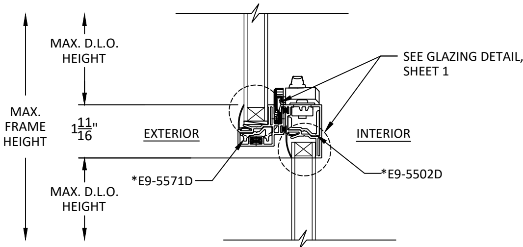
B 5 VERTICAL SECTION INTERLOCK RAIL
