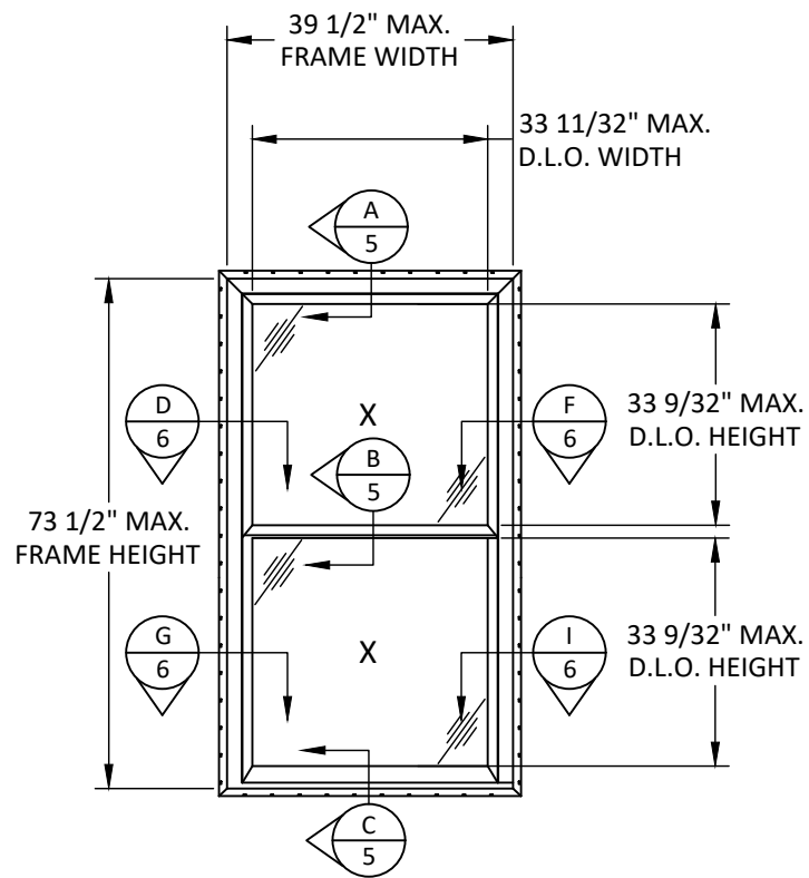
ELEVATION DOUBLE HUNG WINDOW DP50
