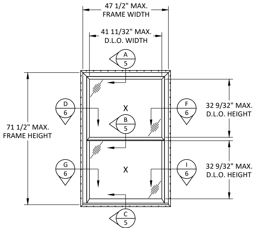
ELEVATION DOUBLE HUNG WINDOW DP35
