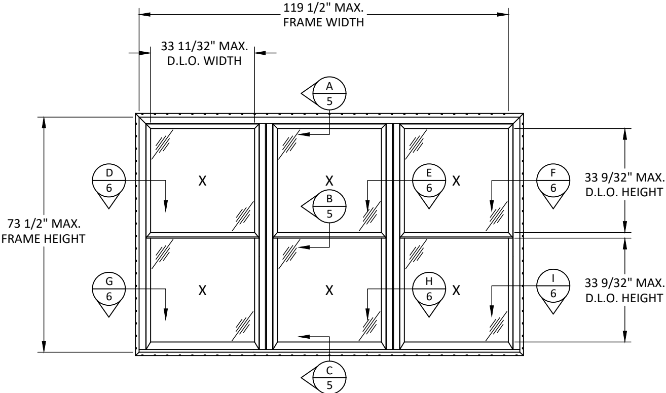
ELEVATION TRIPLE DOUBLE HUNG WINDOW DP35 OR DP50
