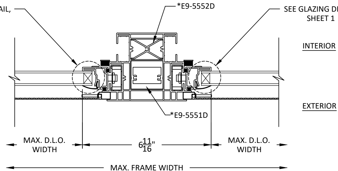
E 6 HORIZONTAL SECTION MULLION
