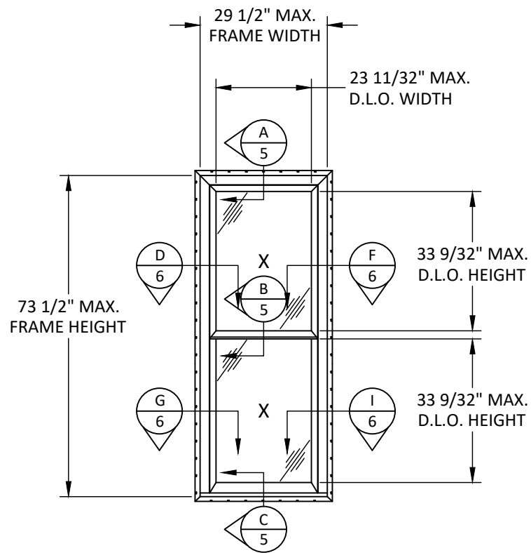
ELEVATION DOUBLE HUNG WINDOW DP50
