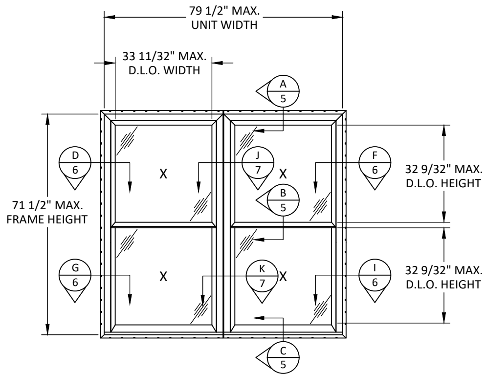
ELEVATION FACTORY MULLED DOUBLE HUNG WINDOW DP50
