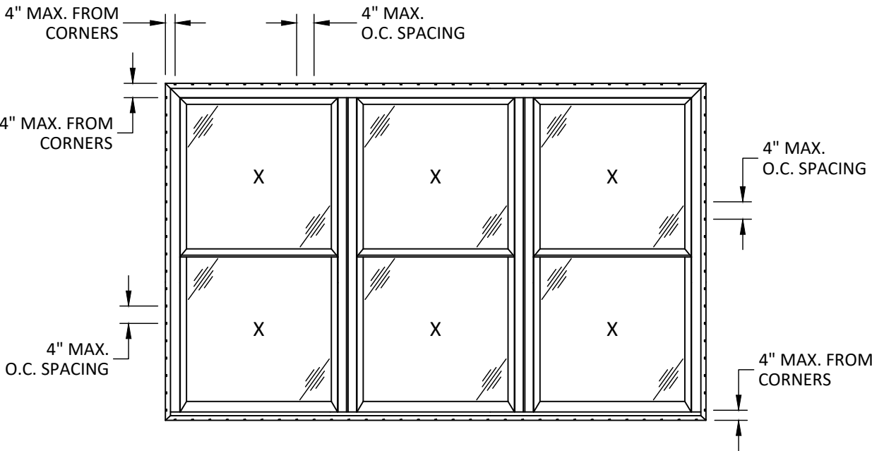
ANCHOR LAYOUT NAILING FIN
