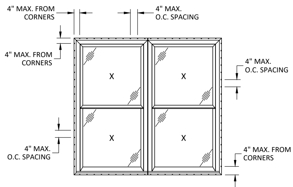
ANCHOR LAYOUT NAILING FIN
