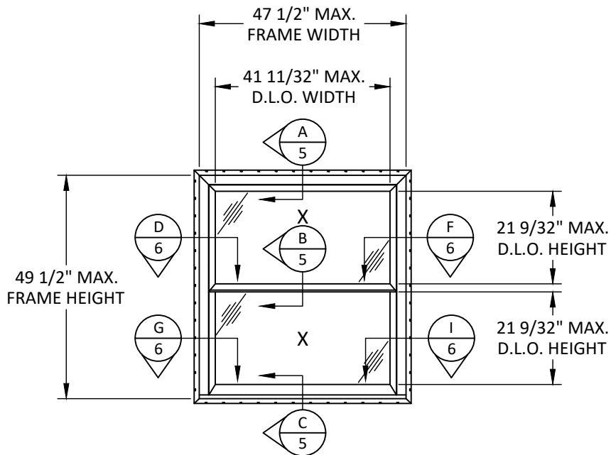
ELEVATION DOUBLE HUNG WINDOW DP50
