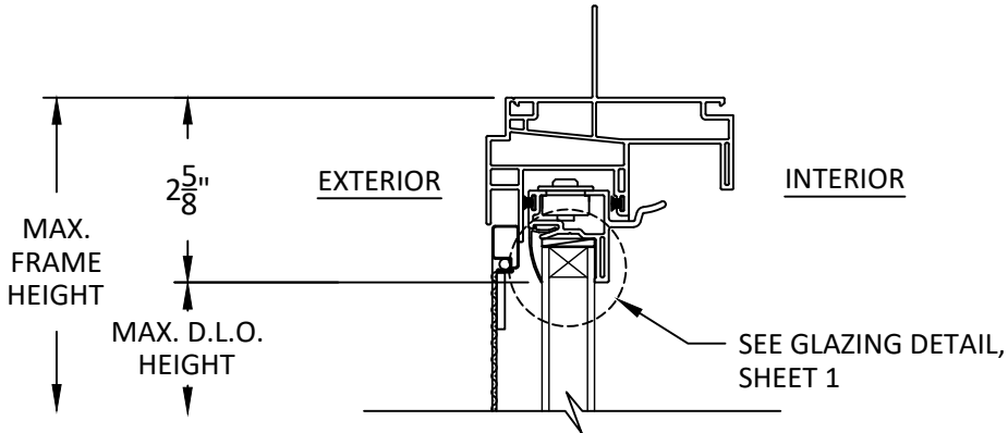
A 5 VERTICAL SECTION HEAD
