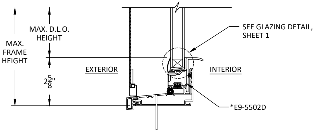
C 5 VERTICAL SECTION SILL
