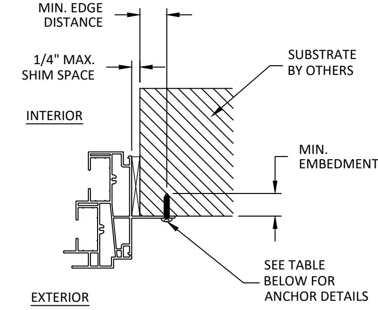
C 8 HORIZONTAL SECTION JAMB INSTALLATION
