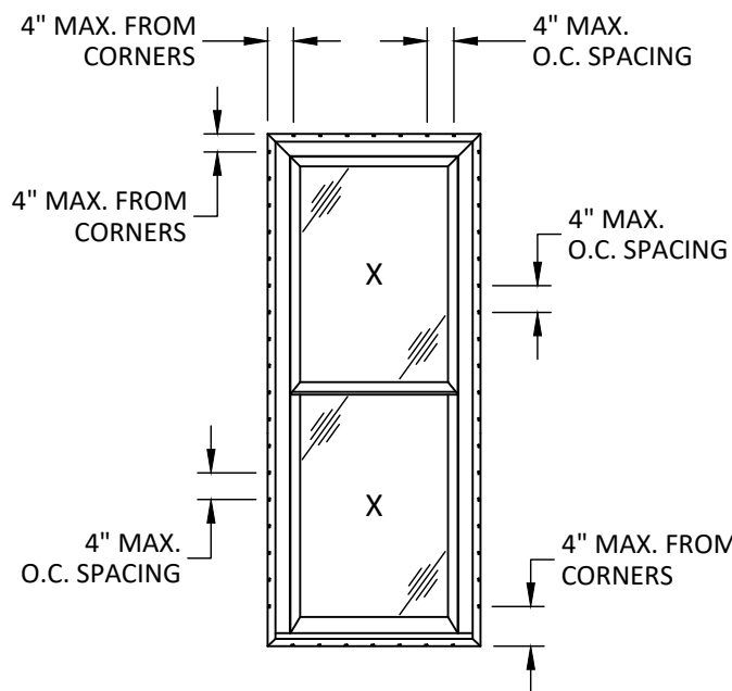
ANCHOR LAYOUT NAILING FIN
